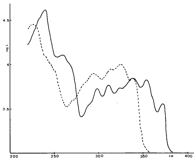
Figure 1. The uv absorption spectra of 4-methyl-dipyrido[1,2- \alpha :3',2'- d ]imidazole in ethanol (—) in ethanol + HCl 10^{-2}M (-----).
